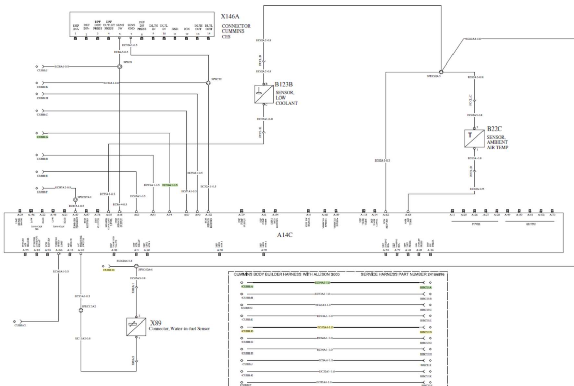
ENGINE CONTROL CUMMINS B SERIES US21 3/3 BODY BUILDER ALLISON 3000
