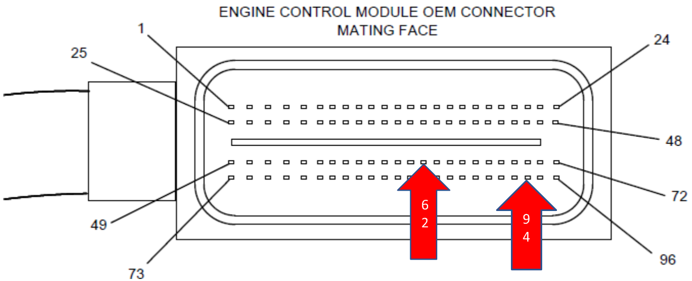
Figure 6 Cummins J2 OEM Connector
